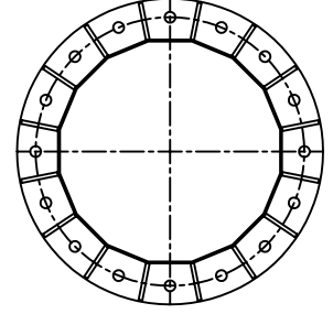
TABAN PLAKASI BASE PLATE
