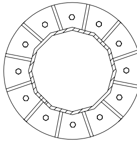
TABAN PLAKASI BASE PLATE
