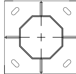
TABAN PLAKASI ANCHOR PLATE
